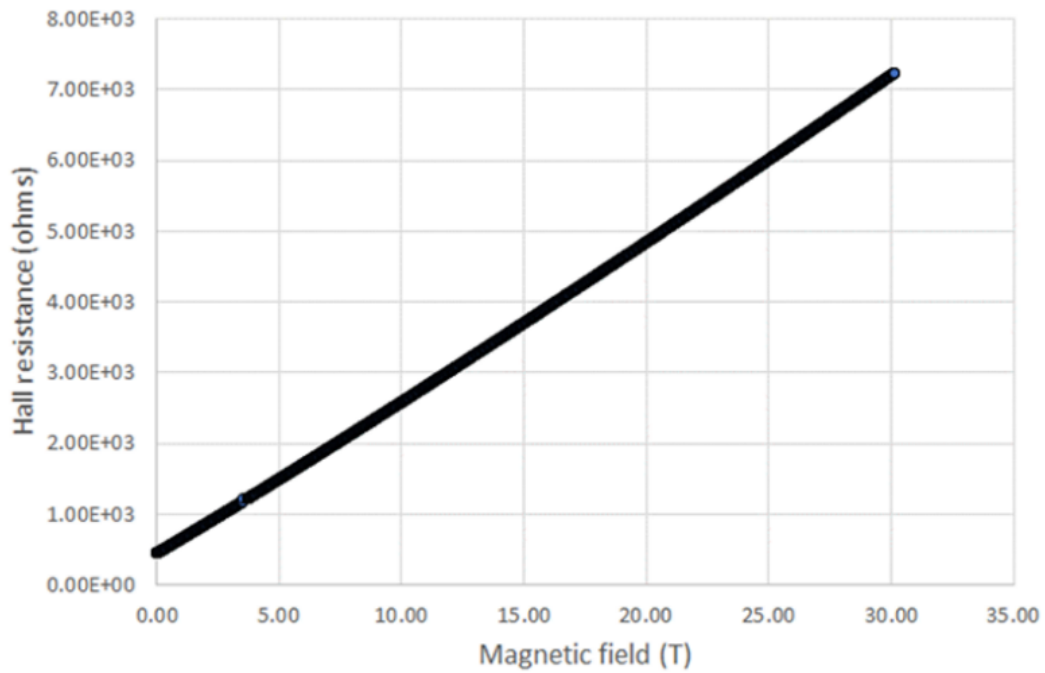
Typical Hall resistance to 30 T at 300 K / 27 °C
