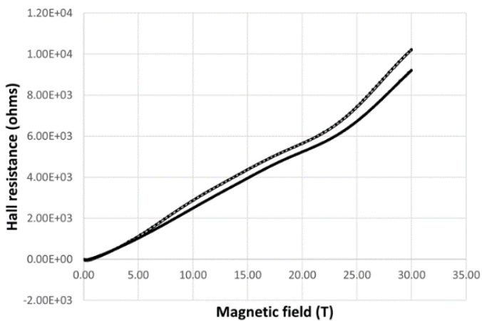
Typical Hall resistance to 30 T at 4 K vs at 1.5 K
